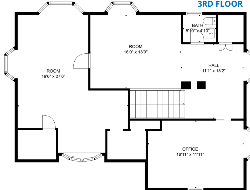
3RD FLOOR
